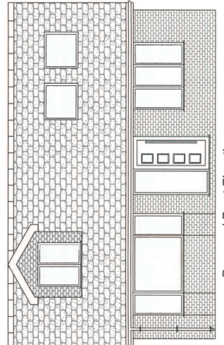
Proposed Front Elevation
